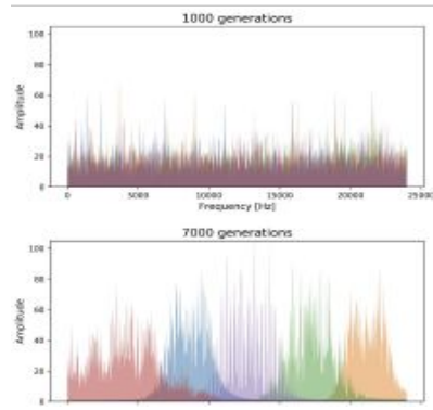
Figure 3: Frequency distributions of agents' voices. The up-per panel shows the distributions at the beginning of the simulation, showing that they are randomly scattered and over-lapped. The lower panel shows the distributions of evolved voices of the elite agents in each species, showing that the distributions converged to specific ranges, and the overlap became smaller than that in upper panel.
