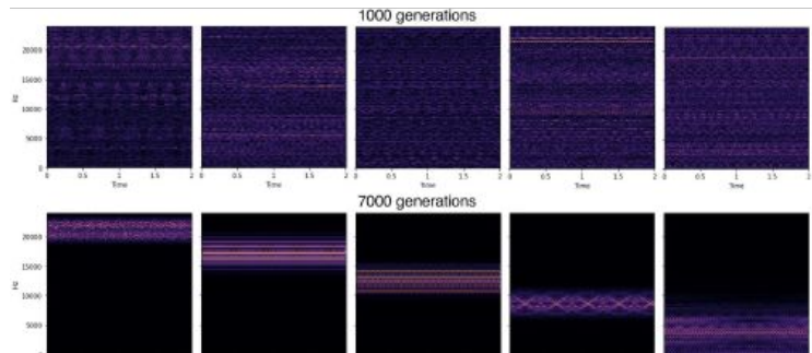
Figure 1: Spectrograms of generated sounds of agents. Figures in the upper panel show the spectrograms of voices of elite agents in each species at the beginning of the simulation (at 1,000 generations), and Figures in the lower panel show the spectrograms of the evolved voices (at 7,000 generations where the fitness values were already converged).
