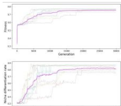
Figure 2: Fitness of the genetic algorithm and the niche differentiation rate increase through generations. The upper panel shows the time series of the fitness, while the lower panel shows the time series of the niche differentiation rate. The thick line represents the mean values of ten simulations, and the dotted line represents the values of each experiment.
